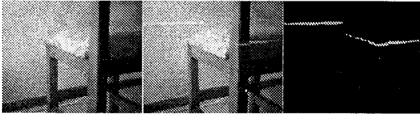
Figure 5: Laser range sensor operation. From left to right: (a) Image from the camera. (b) Image with the laser line generator turned on. (c) Image of (b) - (a)
