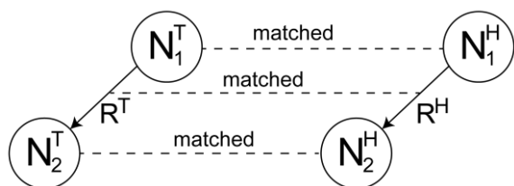
Fig. 3. Matching rule 1
