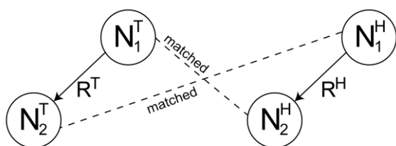
Fig. 4. Matching rule 2
