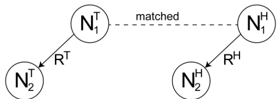
Fig. 7. Matching rule 5
