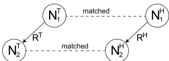
Fig. 5. Matching rule 3
