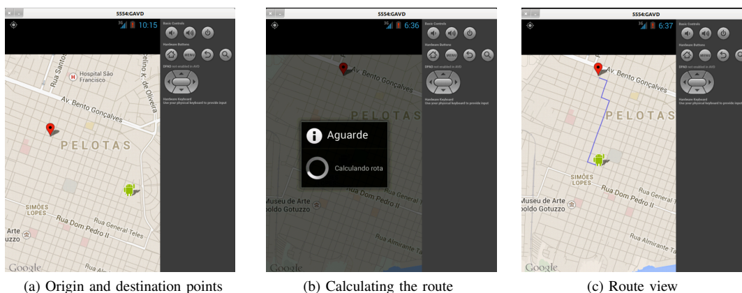
Fig. 1. Prototype Interface
